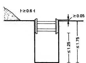
9 Partly secured excavation
